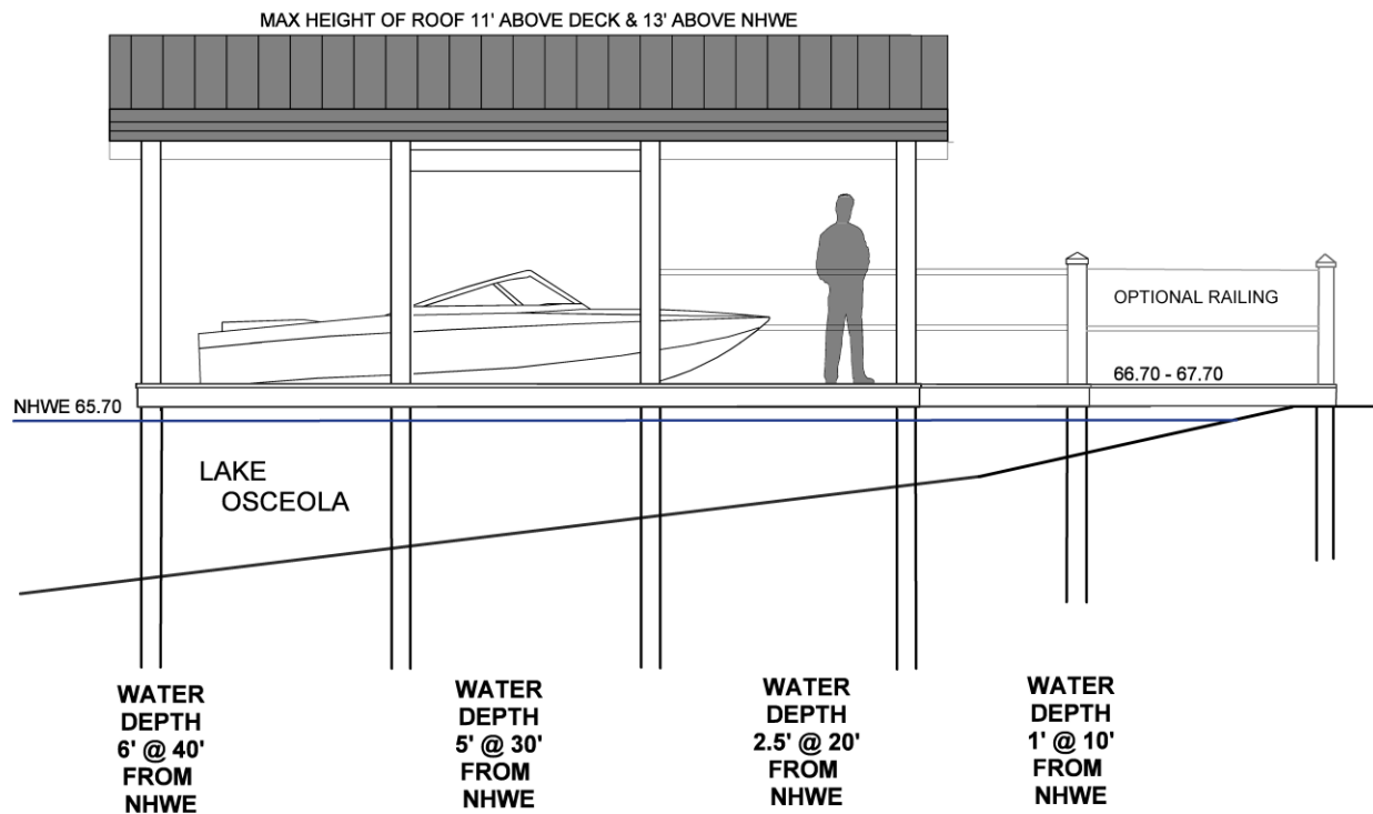
HAGLE BOAT DOCK ELEVATION - 926 PALMER AVENUE, WINTER PARK, FL 32789
