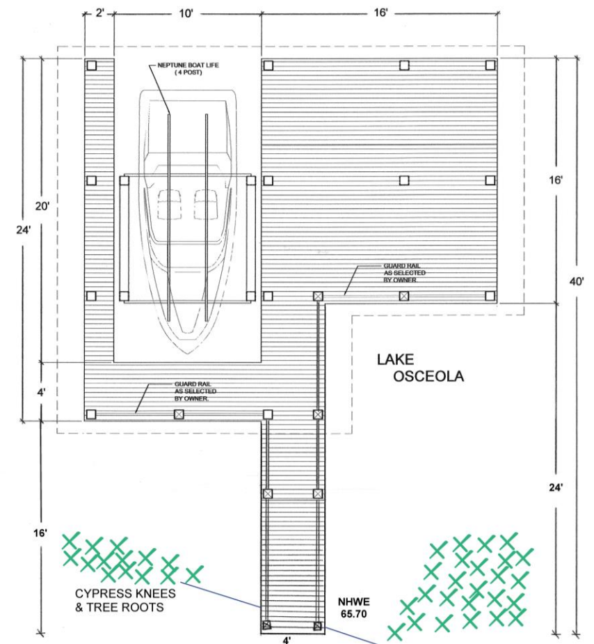
HAGLE BOAT DOCK PLAN VIEW 926 PALMER AVENUE, WINTER PARK, FL 32789
