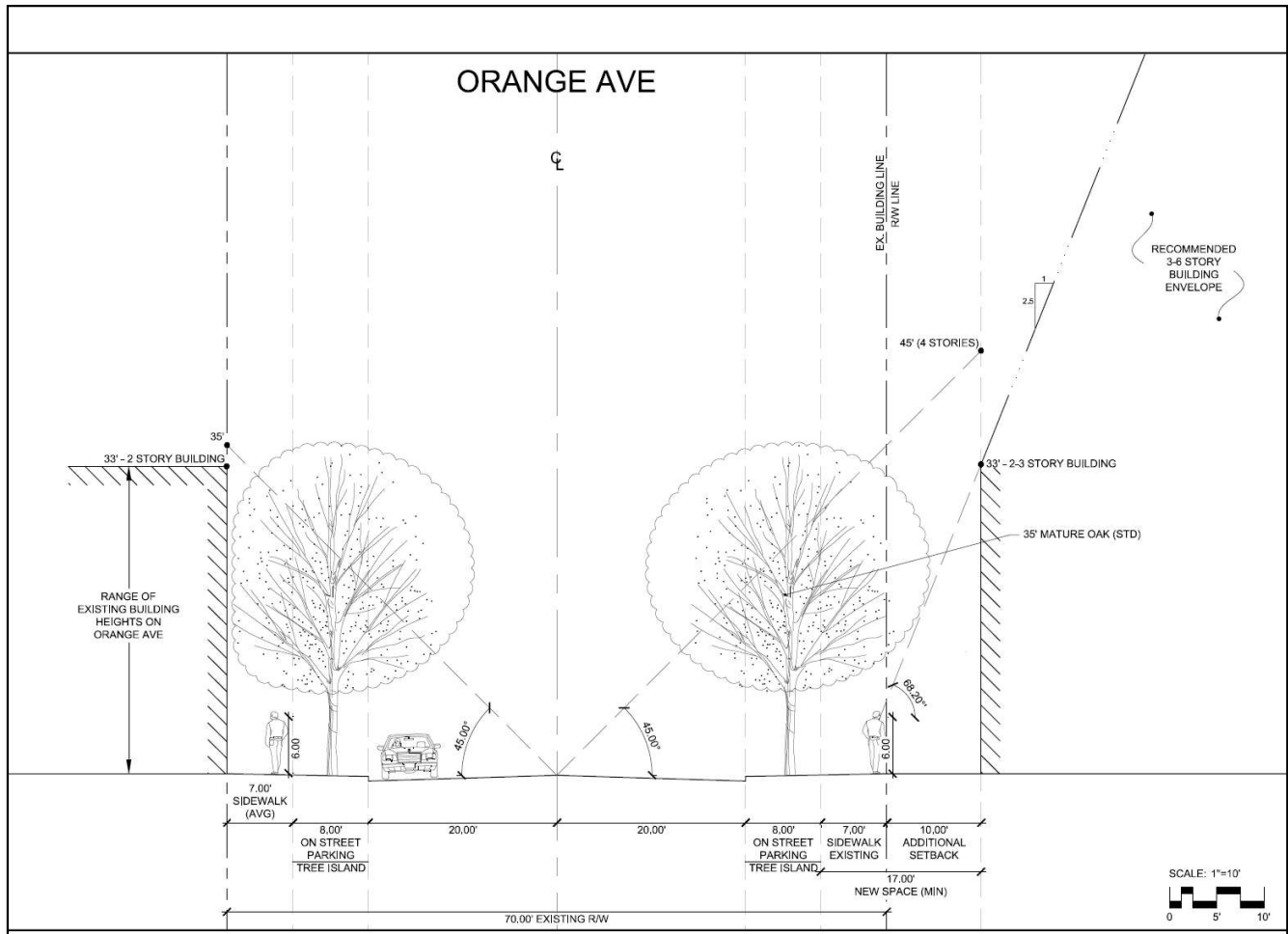
Figure 5 – Typical Cross-Section:
