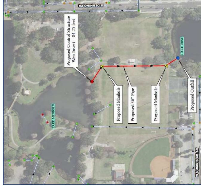
Alternative 2 – New Interconnect Decrease in peak stage (100 yr): 0.05 ft Estimated cost: $172,378
