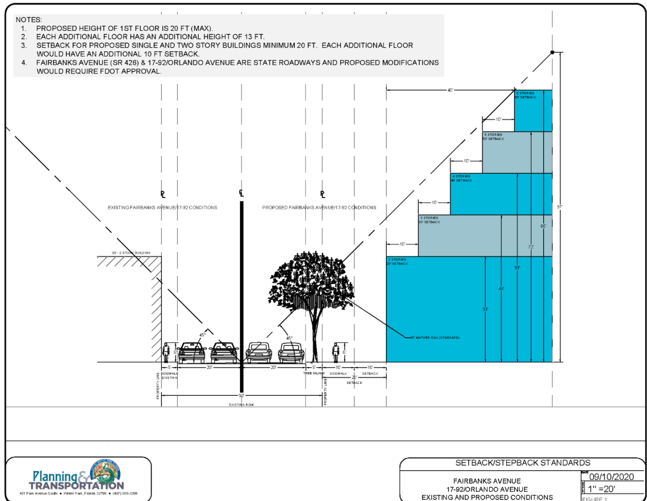
Figure 2 – FDOT Roadway Setback/Stepbacks (17-92 & Fairbanks): Change floor to ceiling height to match code. Change from state roads to all roads for 10 ft setback.
