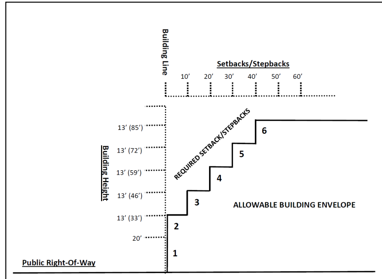
Figure 2 – FDOT Roadway Setback/Stepbacks (17-92 & Fairbanks): Change floor to ceiling height to match code. Change from state roads to all roads for 10 ft setback.
